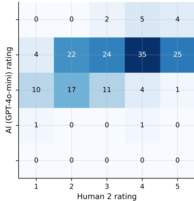
Human 2 vs AI (GPT-4o-mini) \kappa_w = 0.296
