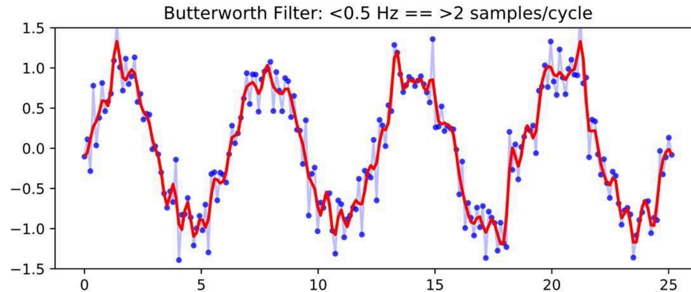
Noisy samples and a smoothed estimate
