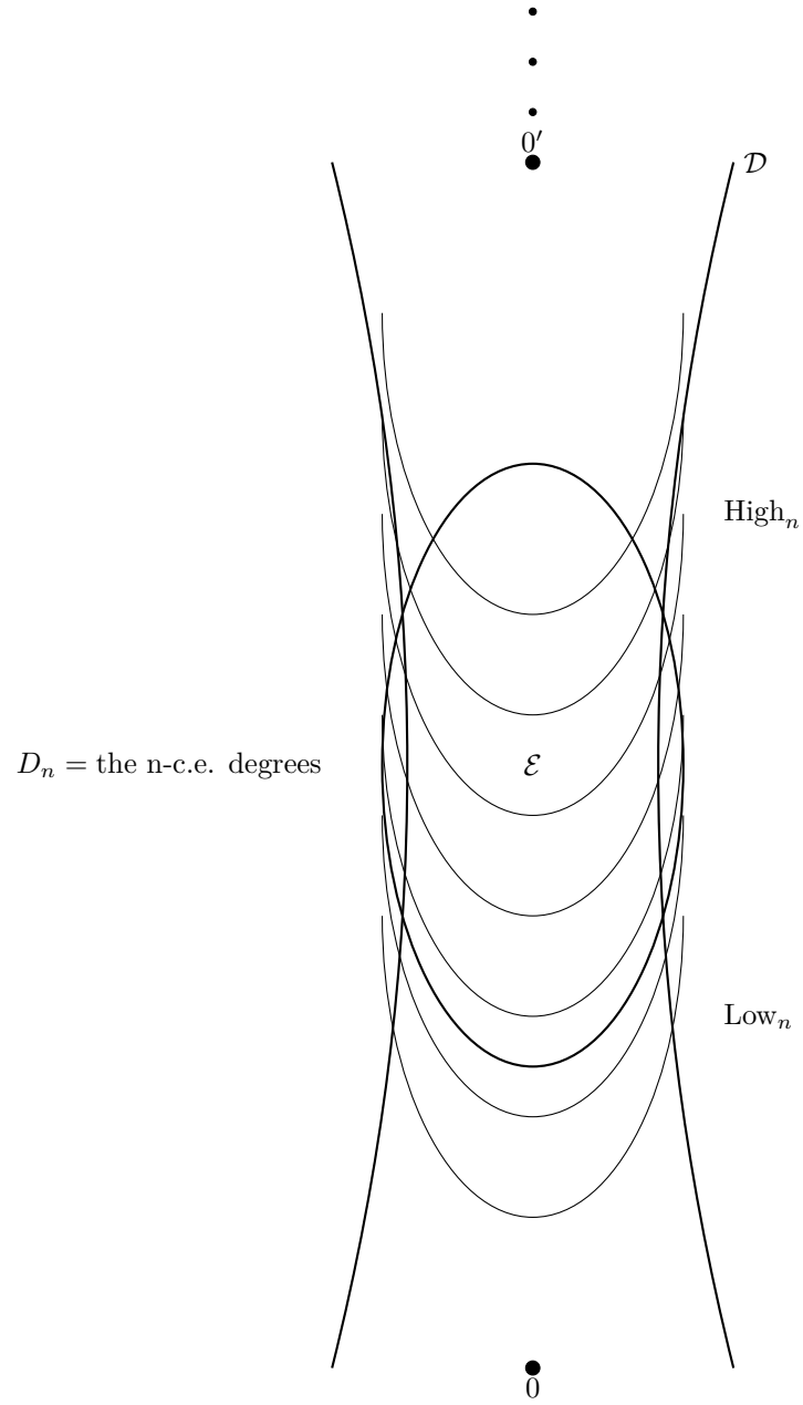
Figure 1.1: Schematic of the n-c.e. hierarchy and degree structure.
