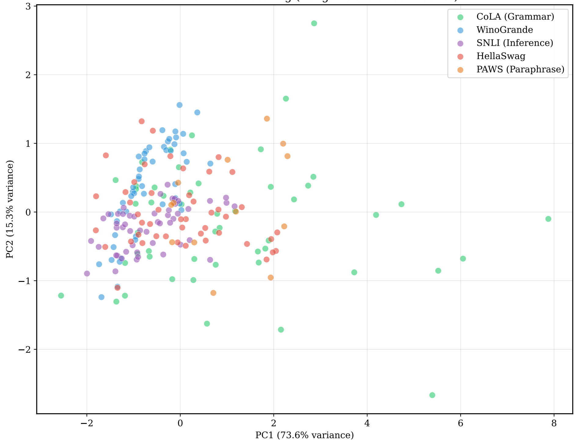
PCA: Domain Clustering (Length-Controlled Metrics)
