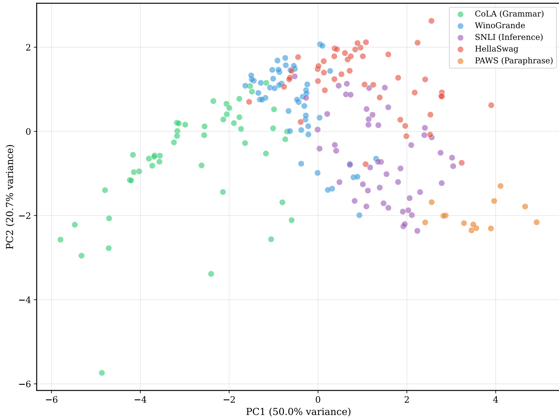
PCA: Domain Clustering on Attribution Features (9 metrics, standardized)
