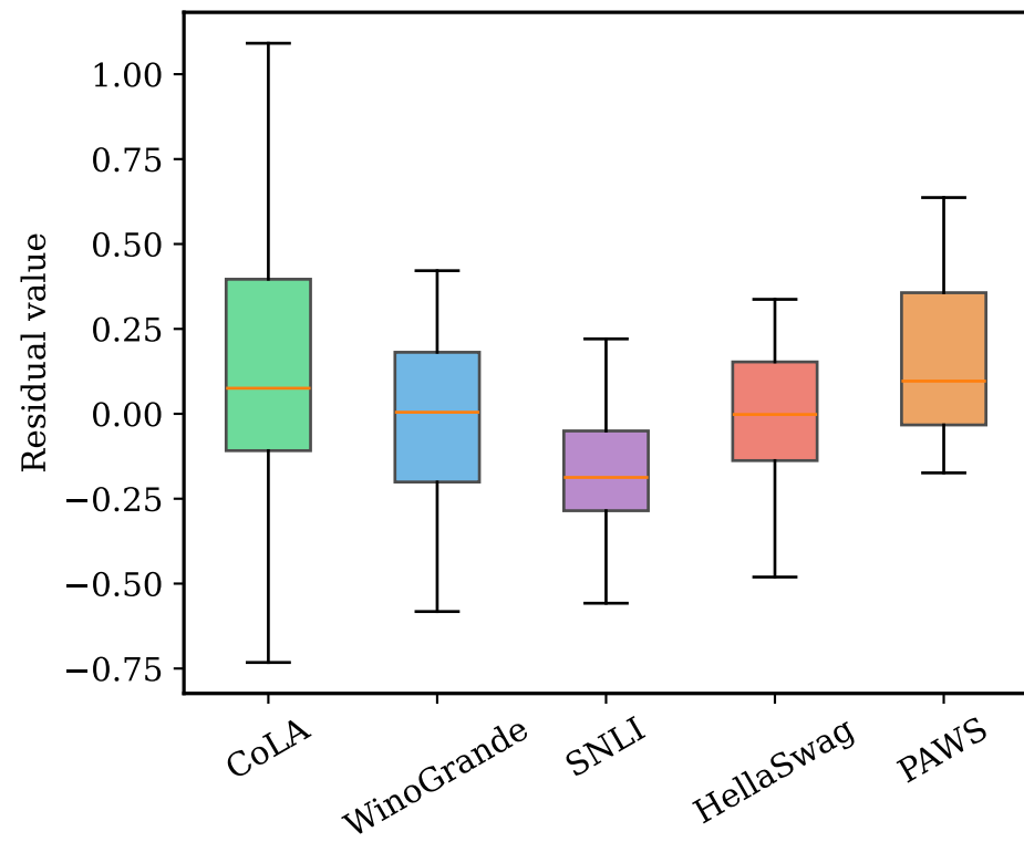
Activation (length-controlled) CoLA vs others: d = 0.64
