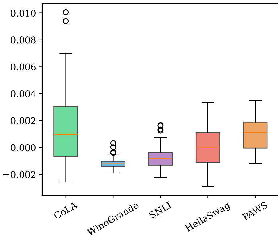
Influence (length-controlled) CoLA vs others: d = 1.08
