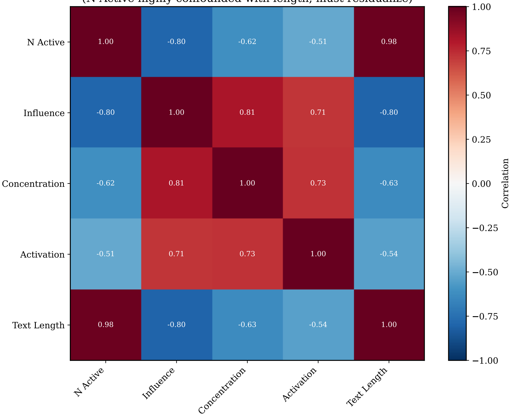
Metric Correlations (N Active highly confounded with length, must residualize)
