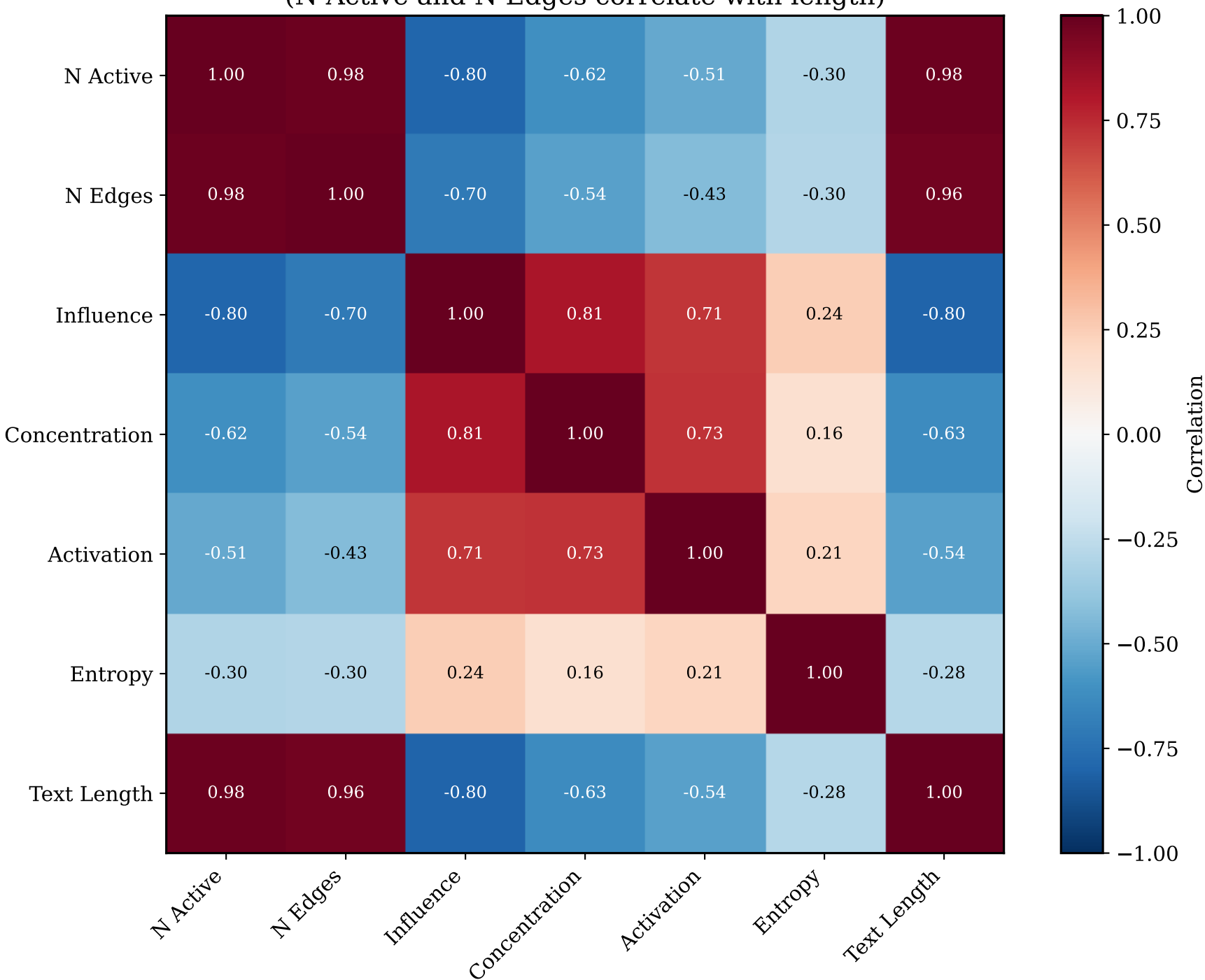
Metric Correlations (N Active and N Edges correlate with length)
