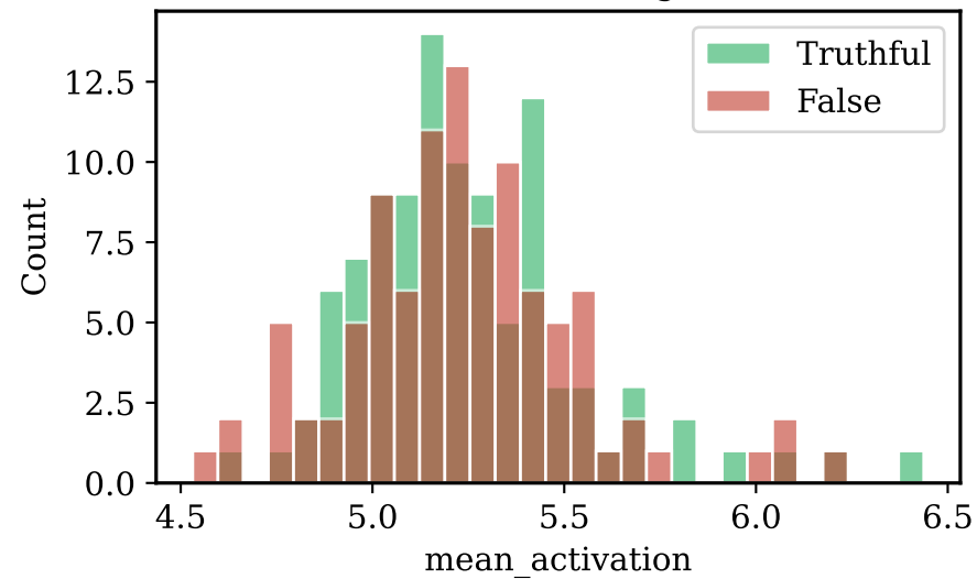
Mean Activation d = 0.042 (no signal)
