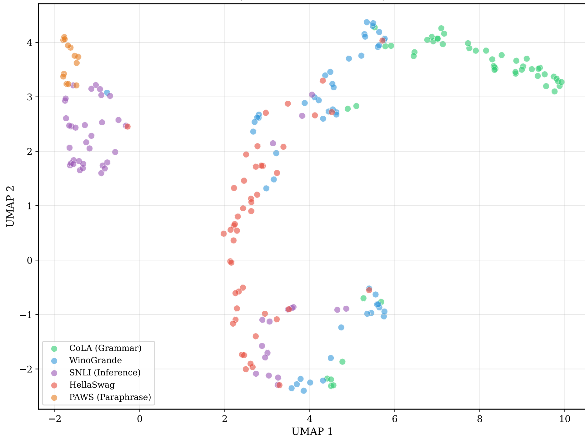
UMAP: Domain Clustering on Attribution Features (9 metrics, standardized)
