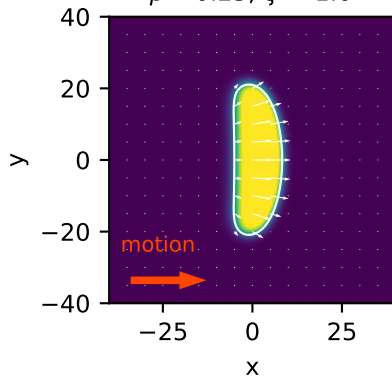
(b) lamellipodium \beta = 0.25, \zeta = -1.0
