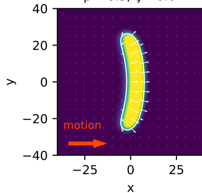
(c) strongly fanned \beta = 0.5, \zeta = 0.0
