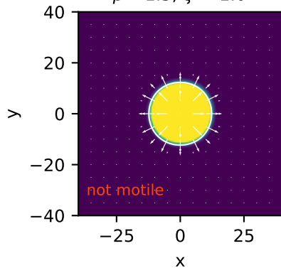
(a) aster / fried egg \beta = 1.5, \zeta = -1.0
