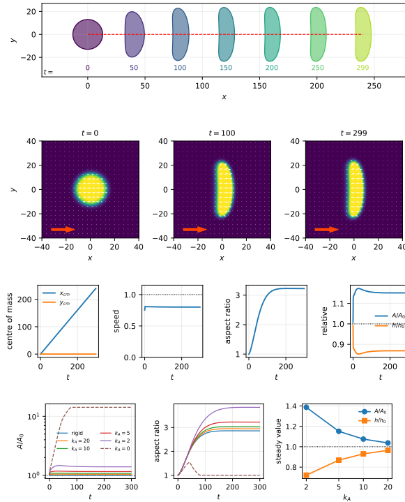
Figure 3: Version 4 crawling (the main result). (a) Laboratory-frame outlines coloured by time; travel 239.9 at speed 0.801. (b) \phi at t = 0, 100, 299 (red arrow: mean \mathbf{P} ). (c) x_{\text{cm}} (linear), speed (0.801), aspect ratio ( \rightarrow 3.2 ), A/A_0 and h/h_0 . (d) Soft volume: A/A_0(t) and aspect ratio for several k_A ; k_A = 0 inflates \sim 14\times .
