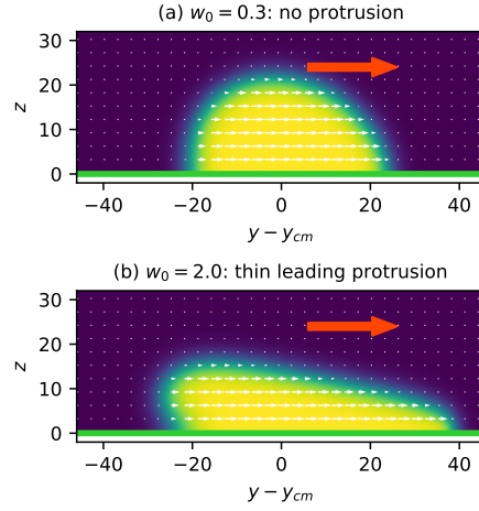
Figure 1: Version 2, vertical slice, wall at z = 0 (green). The two runs differ only in w_0 . (a) w_0 = 0.3 : hemispherical cap. (b) w_0 = 2.0 : thin leading protrusion. White arrows: \mathbf{P} . Volume error 10^{-16} .
