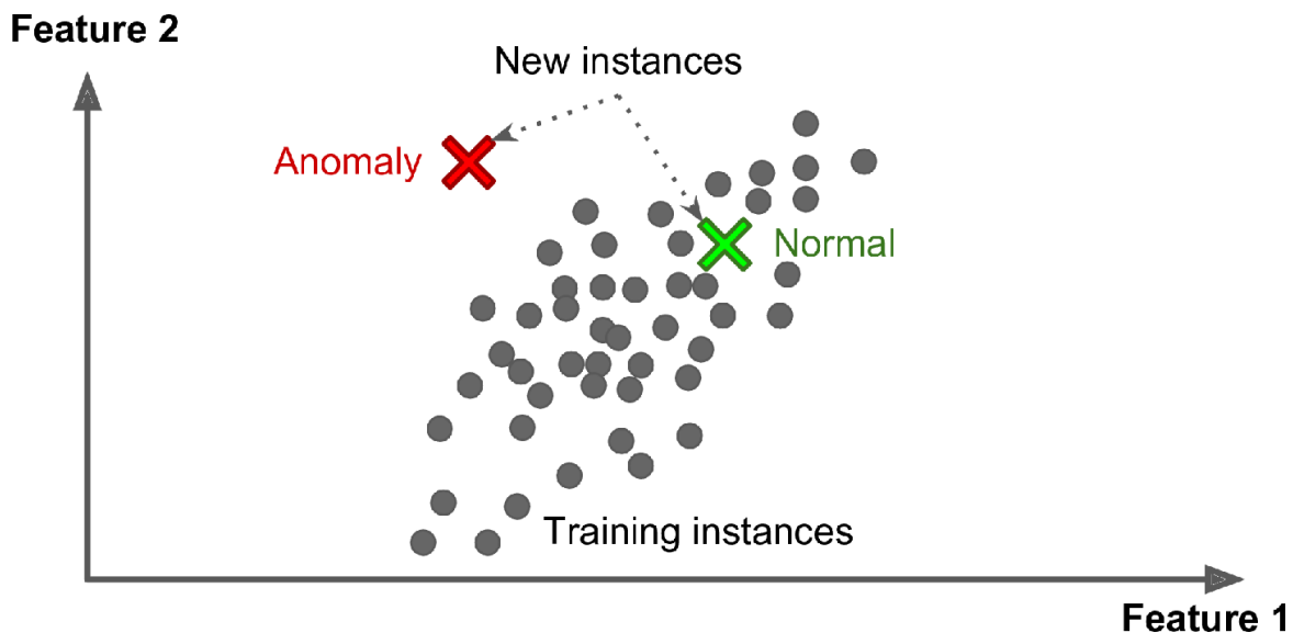
Figure 1-10. Anomaly detection
