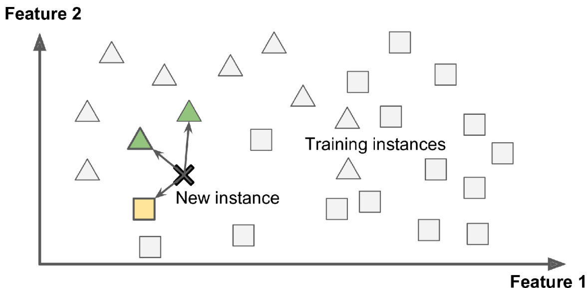
Figure 1-15. Instance-based learning
