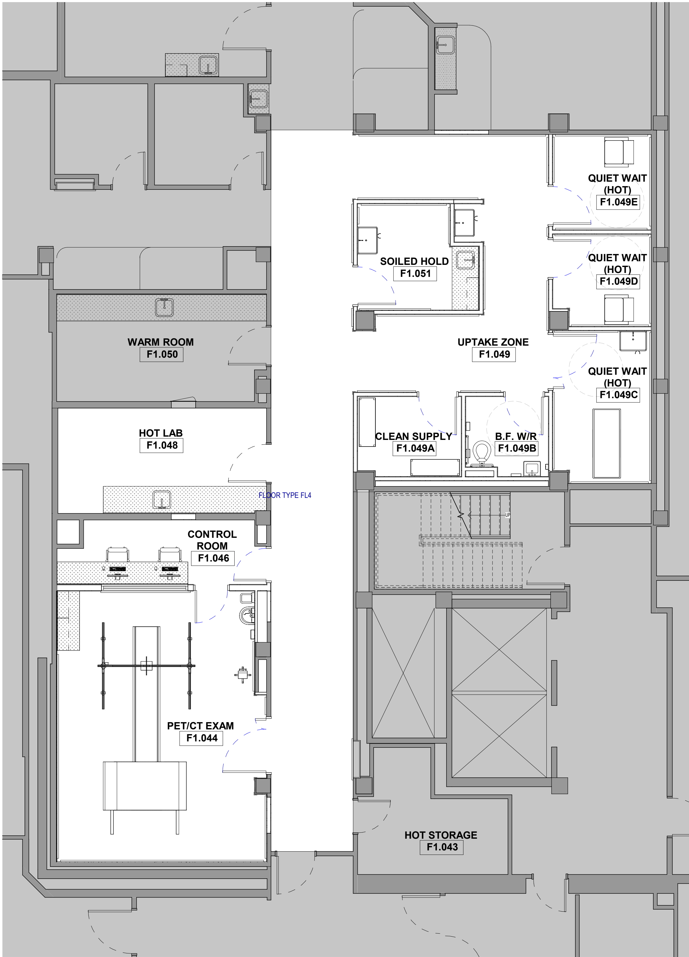
PROPOSED LEVEL 1 FLOOR PLAN
