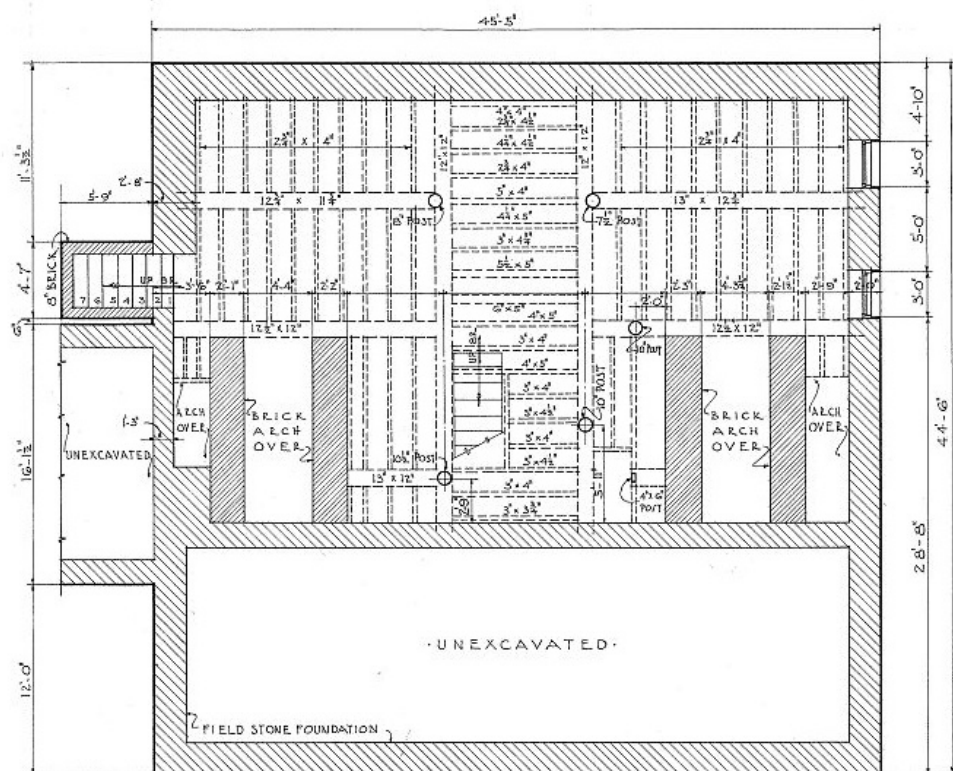
PLAN OF BASEMENT
