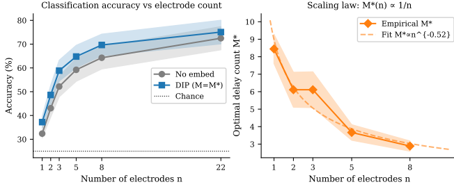
Fig. 3. Left: mean accuracy ( \pm SEM) vs. electrode count for no-embed and DIP. Right: empirical optimal M^*(n) with power-law fit; both consistent with Takens’ bound.
