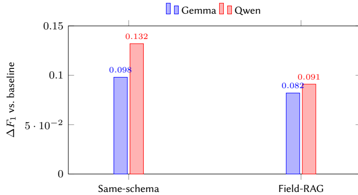
Figure 7: Schema-RAG F_1 gain over the baseline by retrieval route. Field-RAG includes the 99 fallback instances with complete field-embedding diagnostics.
