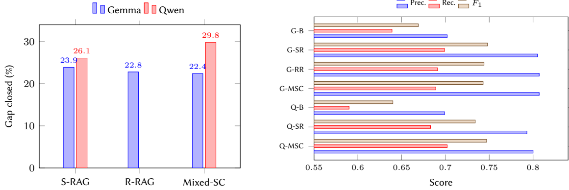
Figure 6: Aggregate result views. Left: fraction of model-specific baseline F_1 gap closed by each non-baseline run. Right: precision, recall, and F_1 by model-pipeline pair. Abbreviations: G/Q = Gemma/Qwen, B = baseline, SR = Schema-RAG, RR = Reasoned-RAG, MSC = Mixed-SC. Qwen Reasoned-RAG was not available.
