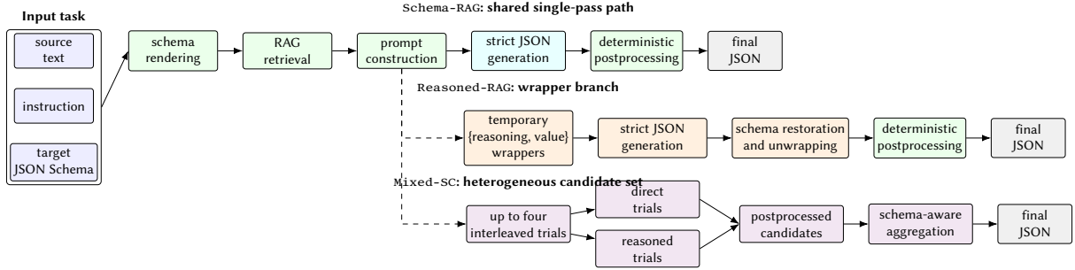
Figure 1: Architecture of the submitted DRILLER pipelines. Schema-RAG follows the shared single-pass path, Reasoned-RAG adds temporary reasoning/value wrappers before restoring the original schema, and Mixed-SC aggregates postprocessed candidates from direct and reasoned trials.
