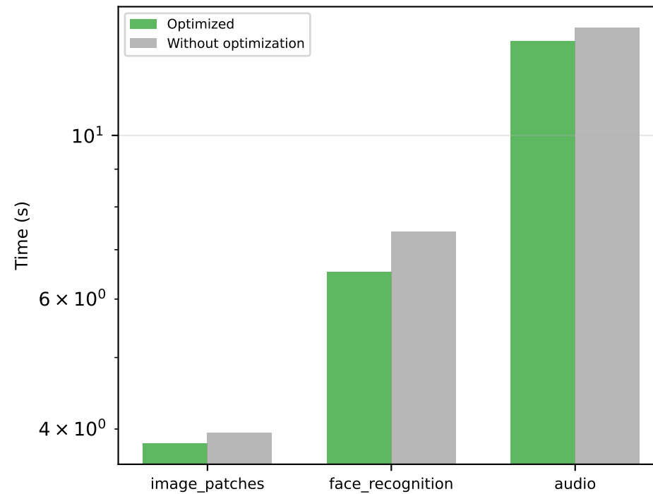
GPU — Gram precomputation
