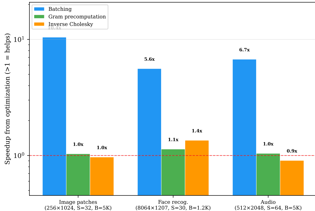
CPU — Ablation: speedup from each optimization
