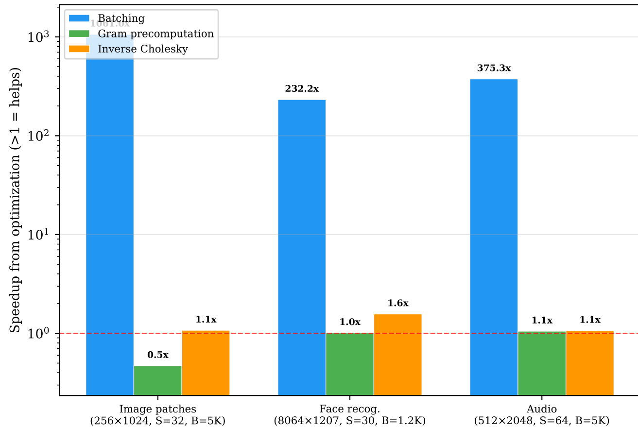
GPU — Ablation: speedup from each optimization
