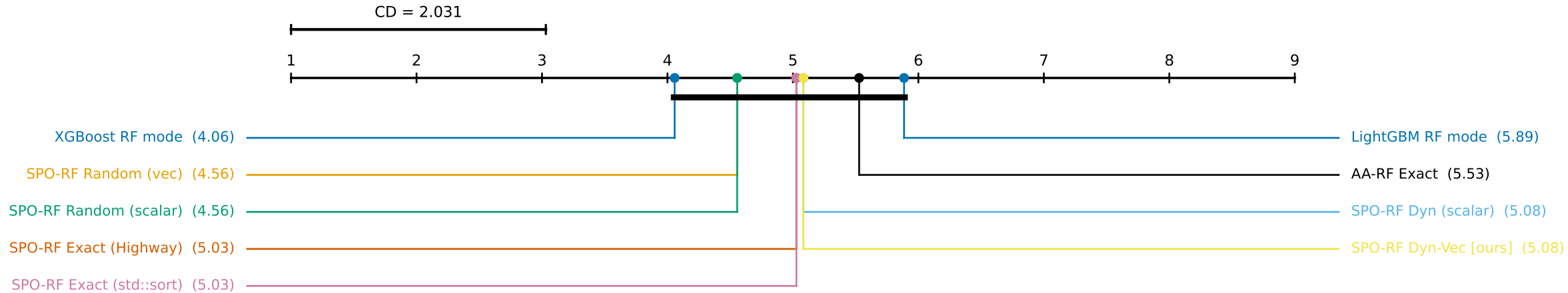
Nemenyi CD diagram -- RF family (AUC) Friedman p=0.1482, n=35 datasets, k=9 methods, CD=2.031 thick bars = not significantly different (Nemenyi, \alpha=0.05 )
