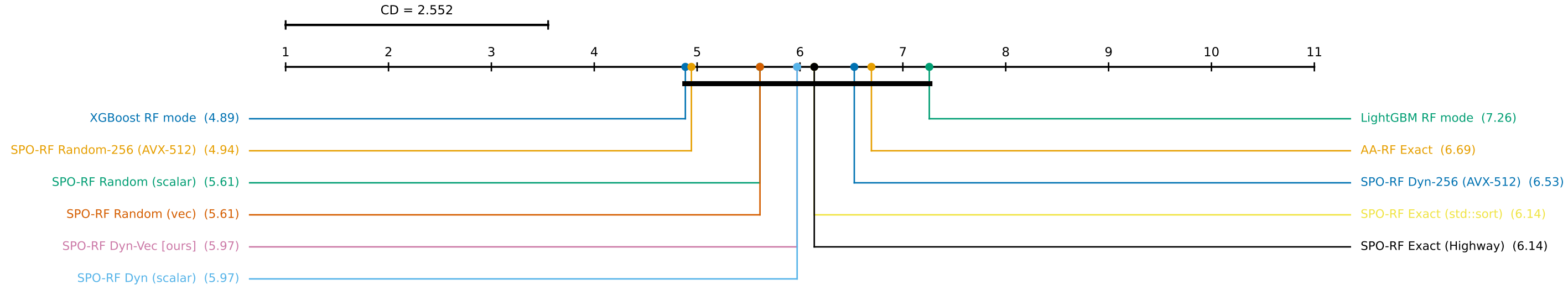
Nemenyi CD diagram -- RF family (AUC) Friedman p=0.06417, n=35 datasets, k=11 methods, CD=2.552 thick bars = not significantly different (Nemenyi, \alpha=0.05 )
