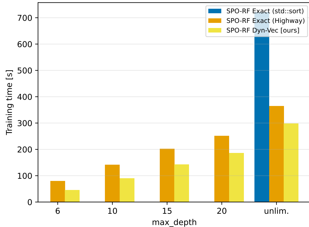
HIGGS (10.5M rows, 240 trees): time by depth
