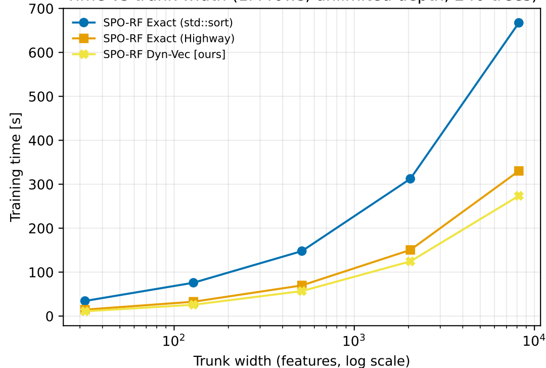
Time vs trunk width (1M rows, unlimited depth, 240 trees)
