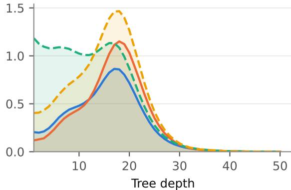
Epsilon, SPO-GBT
