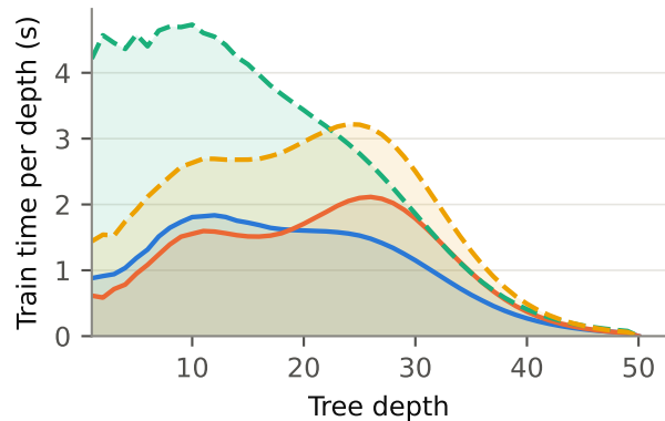
HIGGS, SPO-GBT
