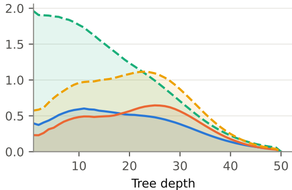
SUSY, SPO-GBT
