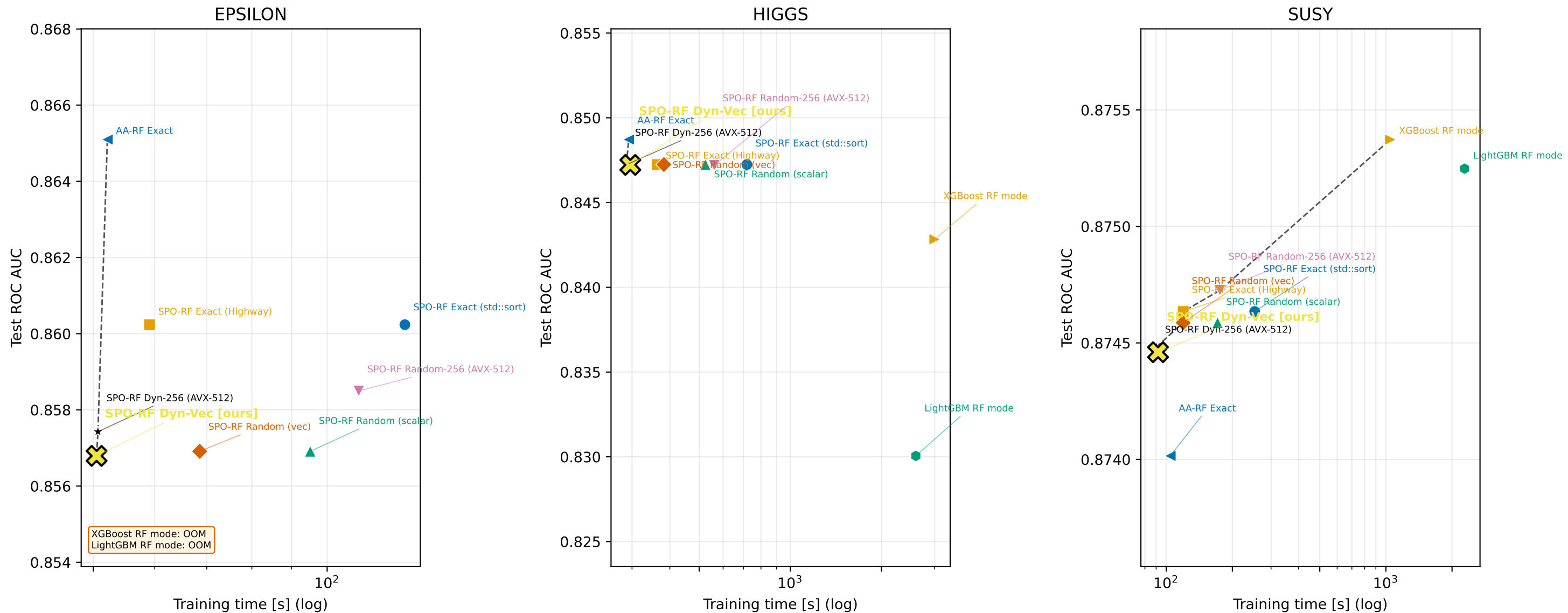
AUC vs training time (train_s) -- huge datasets, RF family only; dashed line = Pareto frontier
