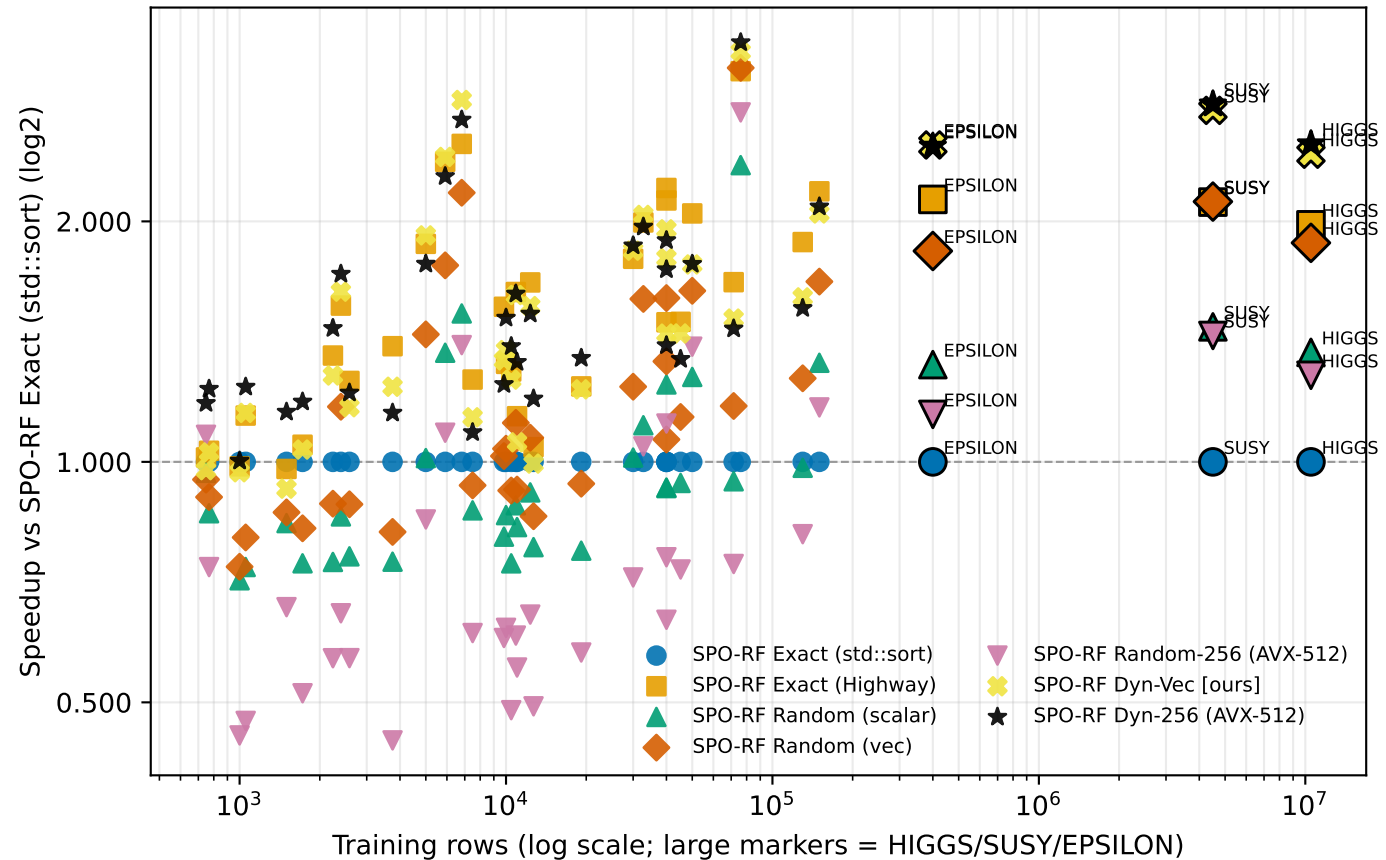
Speedup vs dataset size -- suite + huge datasets, RF family
