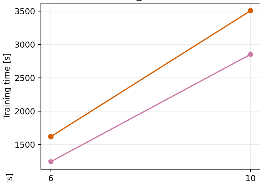
higgs_10500000
