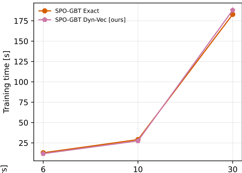
GiveMeSomeCredit
