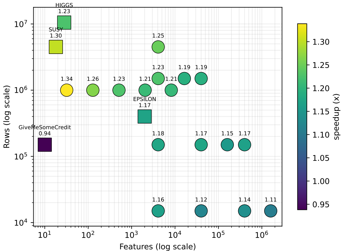
Full-depth RF speedup of SPO Dyn-Vec over SPO-RF Exact (Highway) (240 trees, 48 threads)
