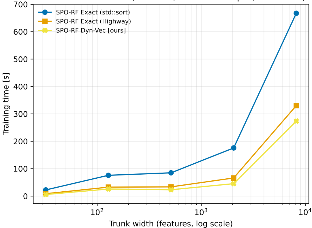
Time vs trunk width (1M rows, unlimited depth, 240 trees)
