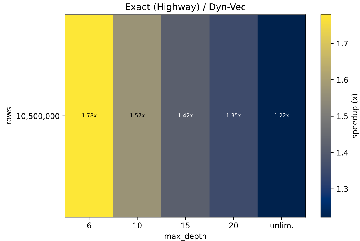
Speedup heatmap -- rows x max_depth (min_examples=1, B1 design)
