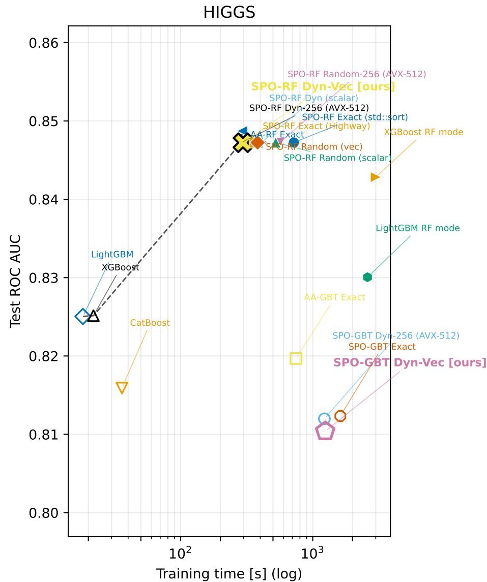
AUC vs training time (train_s) -- huge datasets (single split); dashed line = Pareto frontier
