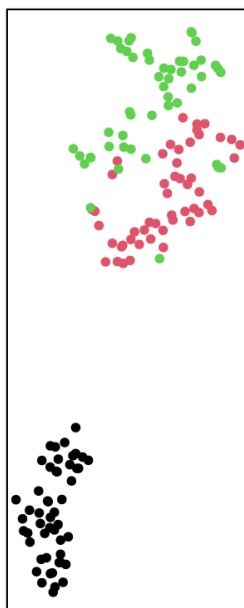
perplexity = 20
