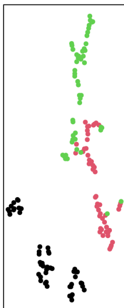
perplexity = 5
