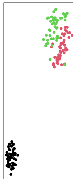
perplexity = 40
