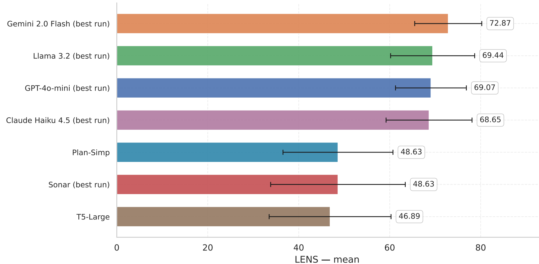
Best run per LLM vs full-dataset baselines (T5-Large, Plan-Simp) LENS
