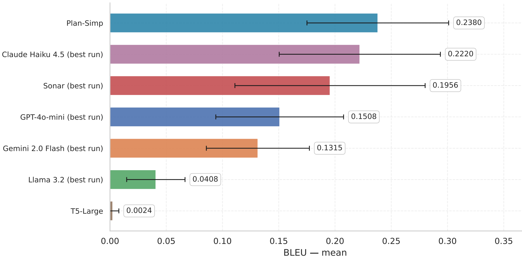
Best run per LLM vs full-dataset baselines (T5-Large, Plan-Simp) BLEU
