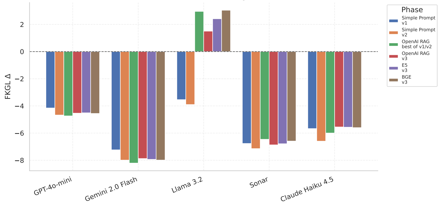
FKGL \Delta (mean over strategies)
