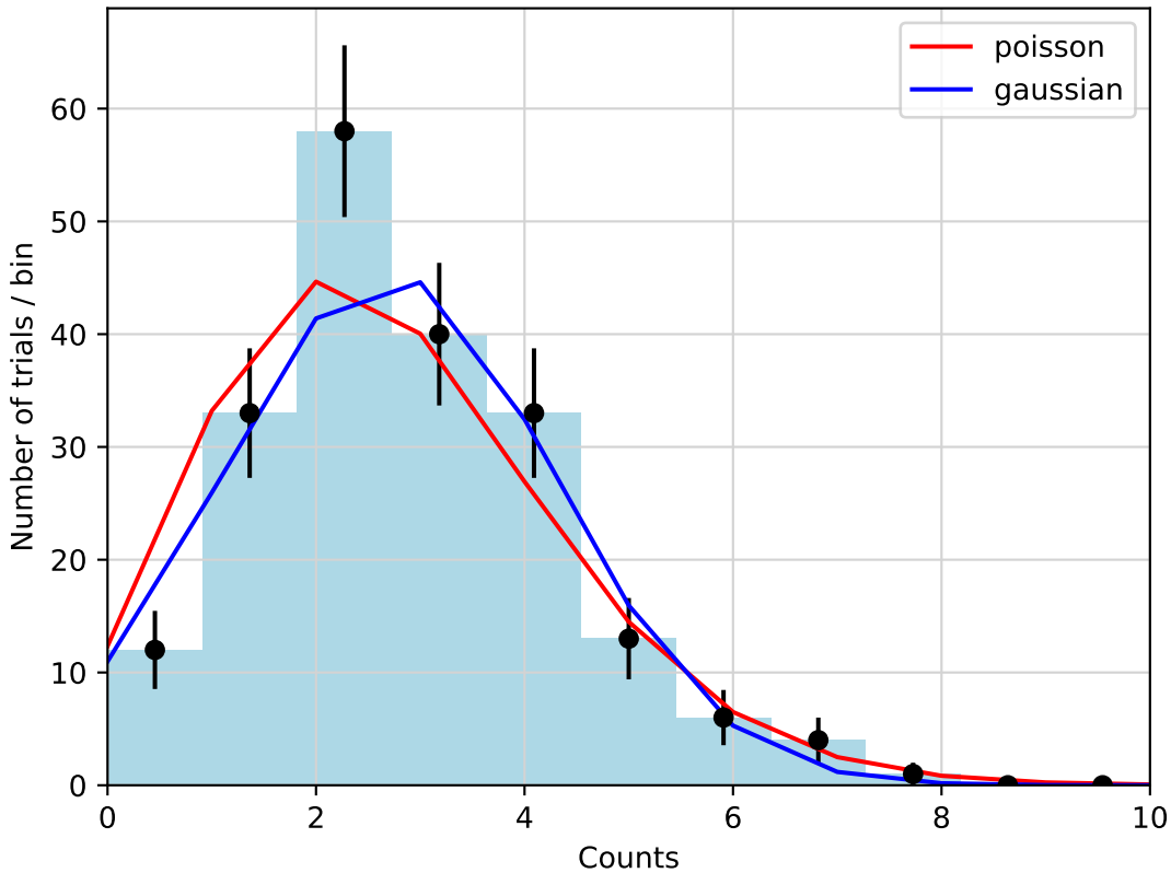
Run01 : poisson and gaussian overlaid
