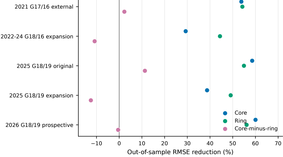
b Component gains transfer inconsistently to the difference
