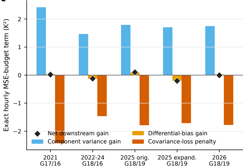
c Covariance loss offsets upstream variance reduction
