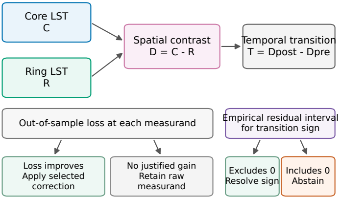
a Loss selection and sign uncertainty determine distinct actions
