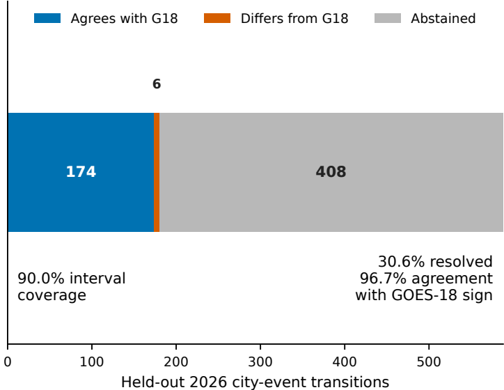
d Residual interval permits selective inference
