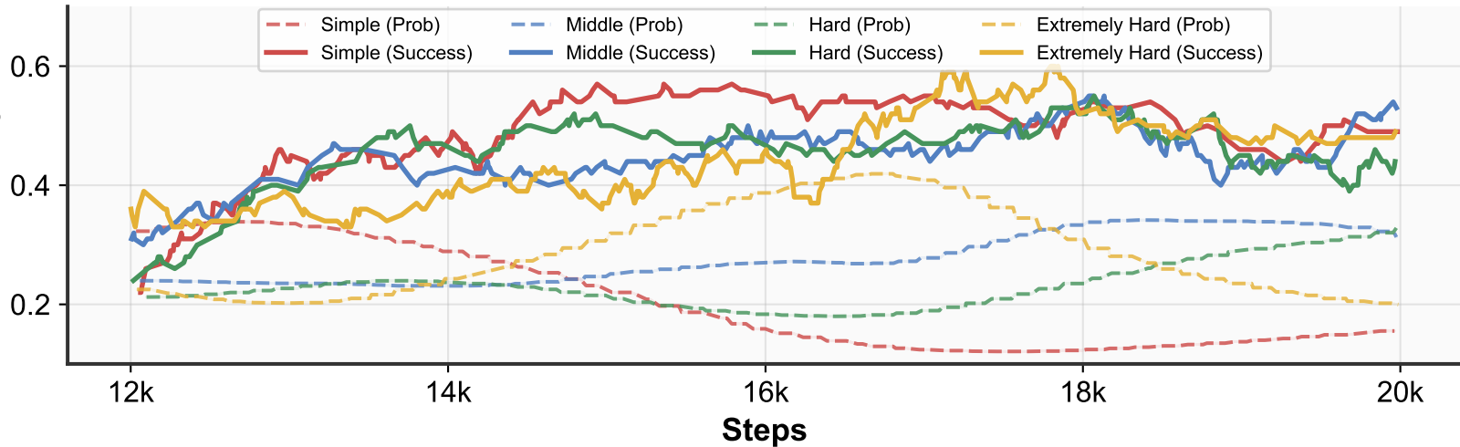
Probability
