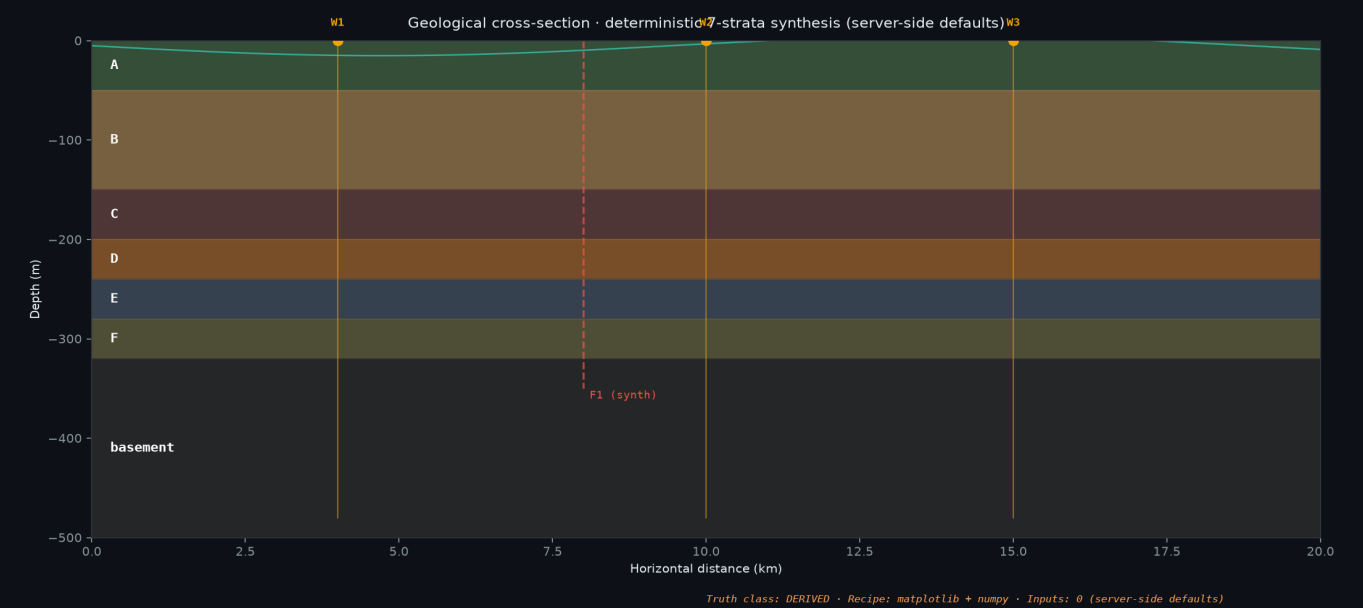
Figure 3 — matplotlib + numpy from documented defaults (7 strata, 3 wells, 1 fault). Inputs = 0 (server-side defaults); data_hash is null by design. A figure with no data hash is a real receipt, not an absence — see FigureAsset v0 nullable data_hash rule.
