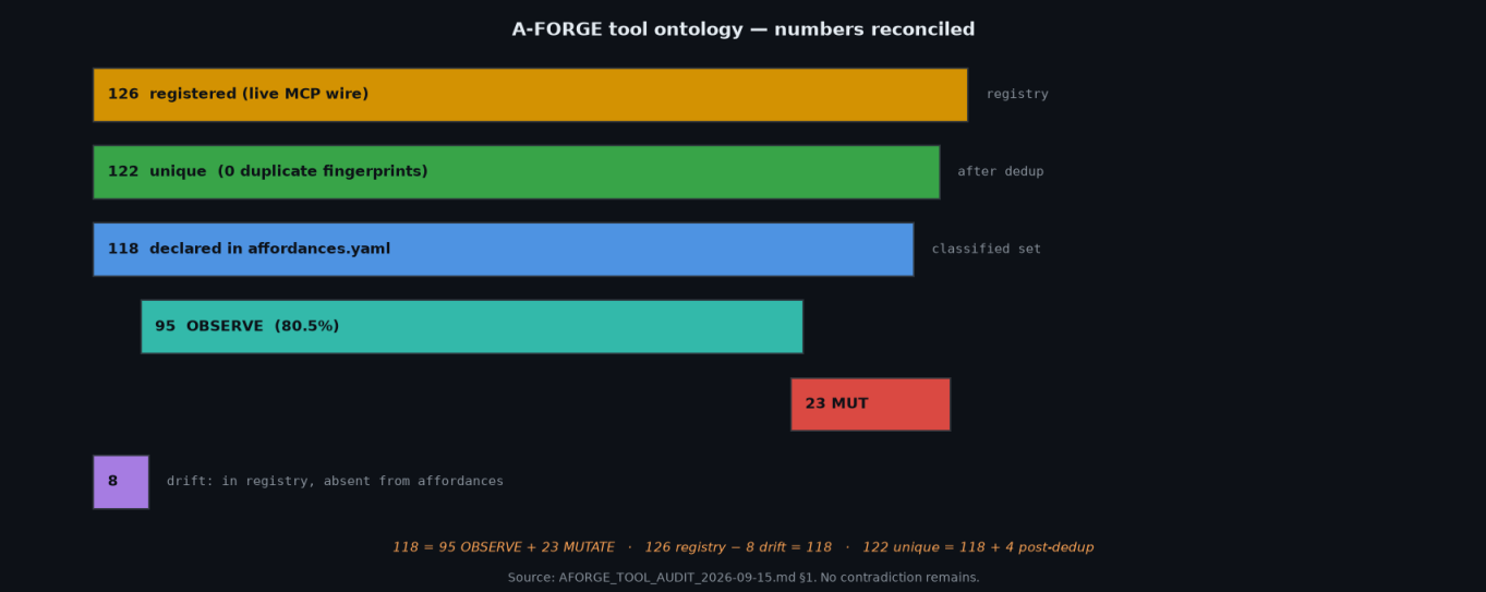
Figure 4 — A-FORGE ontology reconciled. 126 registry – 8 drift = 118 affordance = 95 OBSERVE + 23 MUTATE; 122 unique after fingerprint dedup.
