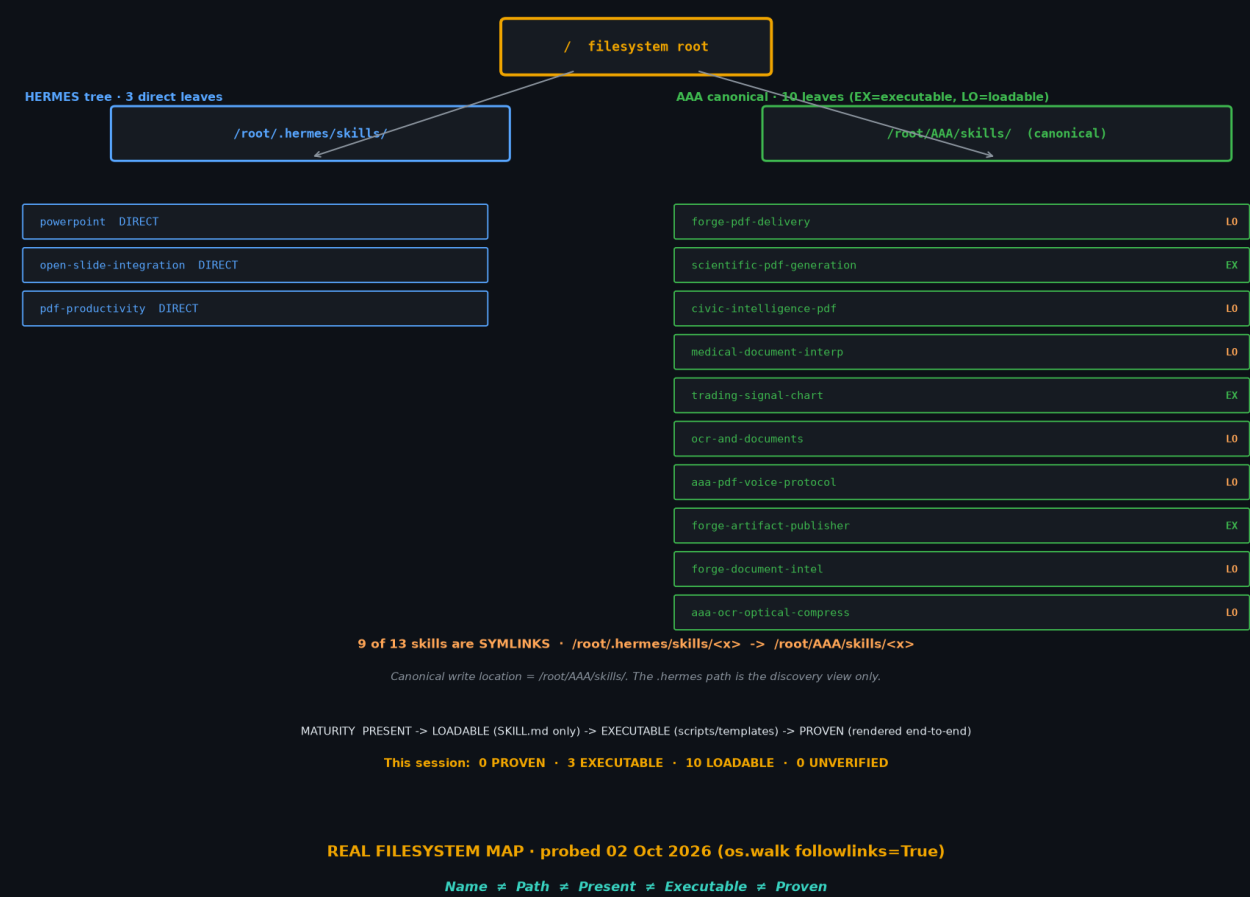
Figure 2 — Every leaf is a real probed path. Where a name resolves to the same physical skill in two places, it is marked DIRECT or symlink rather than duplicated. Canonical write location is /root/AAA/skills/; the /root/.hermes/skills/ path is the discovery view.
