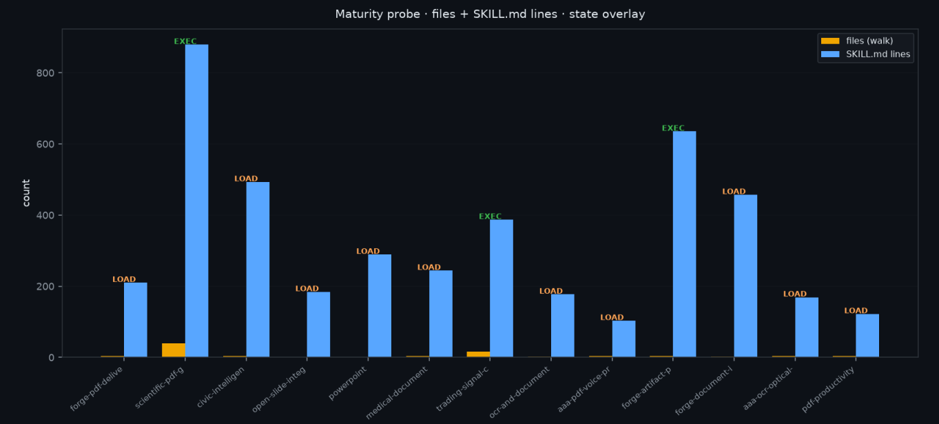
Figure 3 — File count vs SKILL.md length, with state overlay. A long SKILL.md with zero scripts is LOADABLE, not EXECUTABLE.
