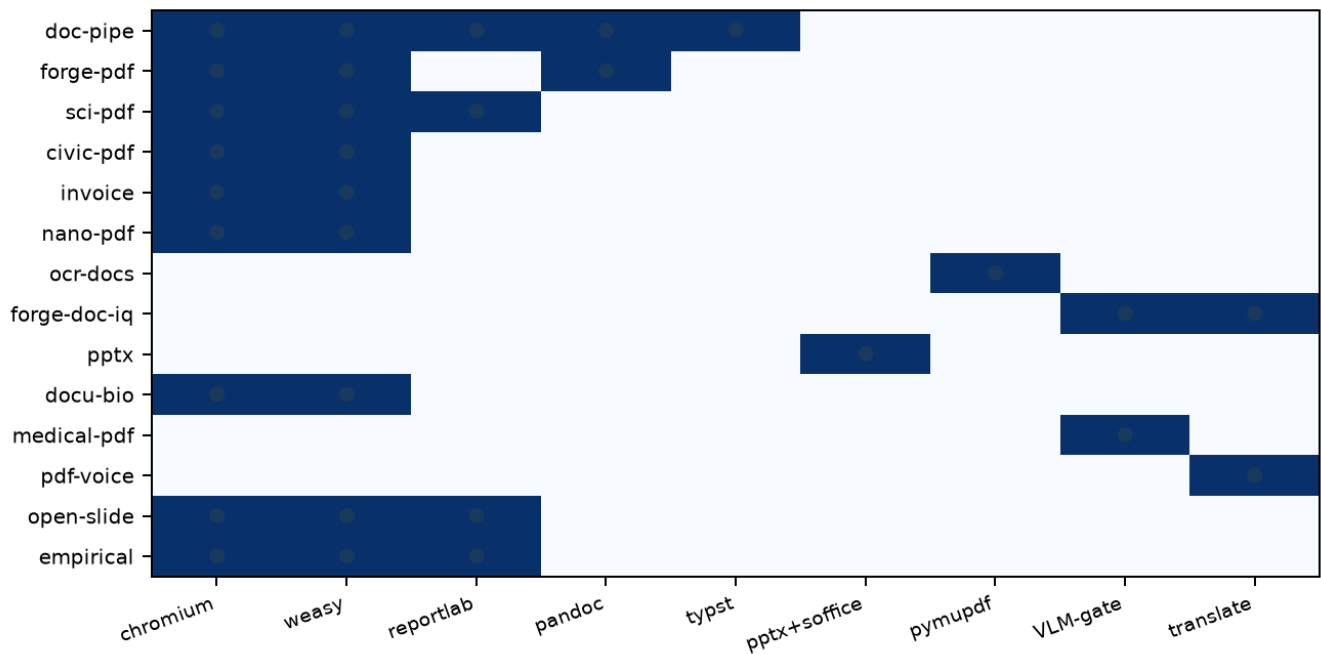
Figure 2 — engine × skill matrix (1 = primary, 0 = unused)
