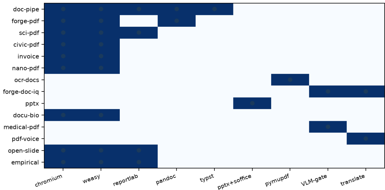
Figure 2 — engine x skill matrix (1 = primary, 0 = unused)
