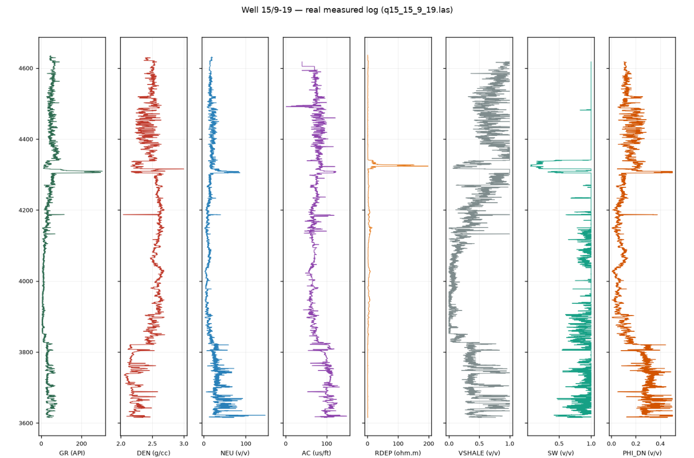
Figure · fig-wellog-real · source=Equinor Volve 15/9-19 LAS (open data) · truth_class=OBSERVATION · render_hash=fe921832ddaf97bb7c597aad2bf3f50f... · data_hash=9f7d0319b815093d ·
