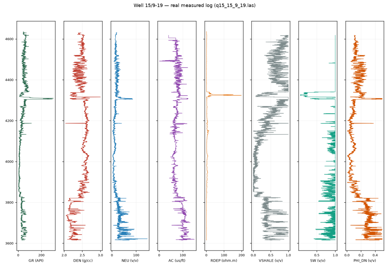
Figure · fig-welllog-real · source=Equinor Volve 15/9-19 LAS (open data) · truth_class=OBSERVATION · render_hash=fe921832ddaf97bb7c597aad2bf3f50f...
