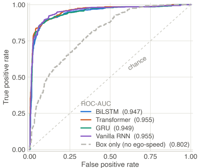
(a) ROC
