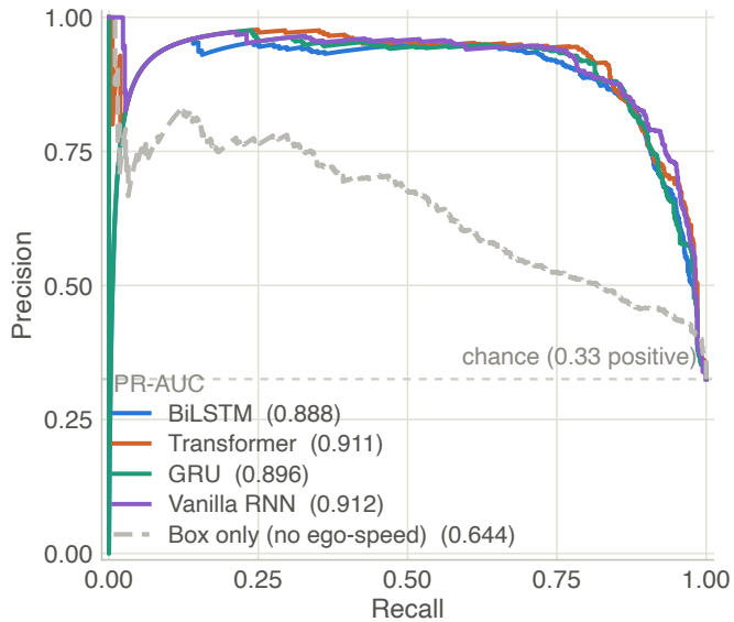
(b) Precision-recall
