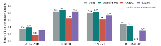
Fig. 2. Leave-one-dataset-out binary F1 (Table III), with the within-dataset reference of 0.907. Instance normalisation — the cheapest adaptation — is the best method on folds A–C; no method helps on fold D, which conflates domain, placement and modality shift.
