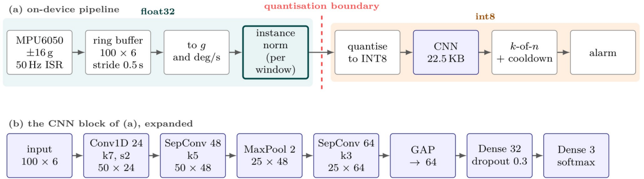
Fig. 1. The deployed system. (a) The on-device pipeline, shaded by numeric domain. Sampling is hardware-timer driven rather than a polled delay, because loop jitter accumulates and shifts window content away from the training distribution. Per-window instance normalisation is deliberately placed on the float side of the quantisation boundary: as a layer inside the graph it is mathematically identical but costs 30.95 points of macro-F1 under INT8 (Section V-F). (b) The network. Separable convolutions and global average pooling hold it to 7,947 parameters; batch normalisation and ReLU follow each convolution, and a flatten in place of the pooling would cost 51,200 parameters in a single layer.
