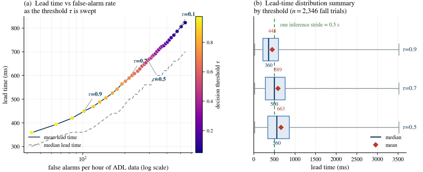
Fig. 3. The central operational trade-off on KFall, pooled over 32 LOSO folds. (a) Mean lead time against false alarms per hour of ADL data as the threshold is swept from 0.05 to 0.975. (b) Lead-time summary at three thresholds (box: min-Q1-median-Q3-max; diamond: mean); the dotted line marks one 0.5 s inference stride. Because the mean lead of 663 ms at threshold 0.5 is barely longer than a stride, any k-of-n debouncing consumes most of the lead time it is meant to protect, and the mean overstates the typical case, so the distribution is reported rather than the mean alone.
