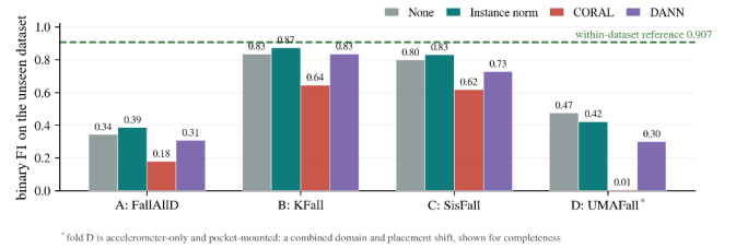
Fig. 2. Leave-one-dataset-out binary F1 (Table III), with the within-dataset reference of 0.907. Instance normalisation — the cheapest adaptation — is the best method on folds A–C; no method helps on fold D, which conflates domain, placement and modality shift.
