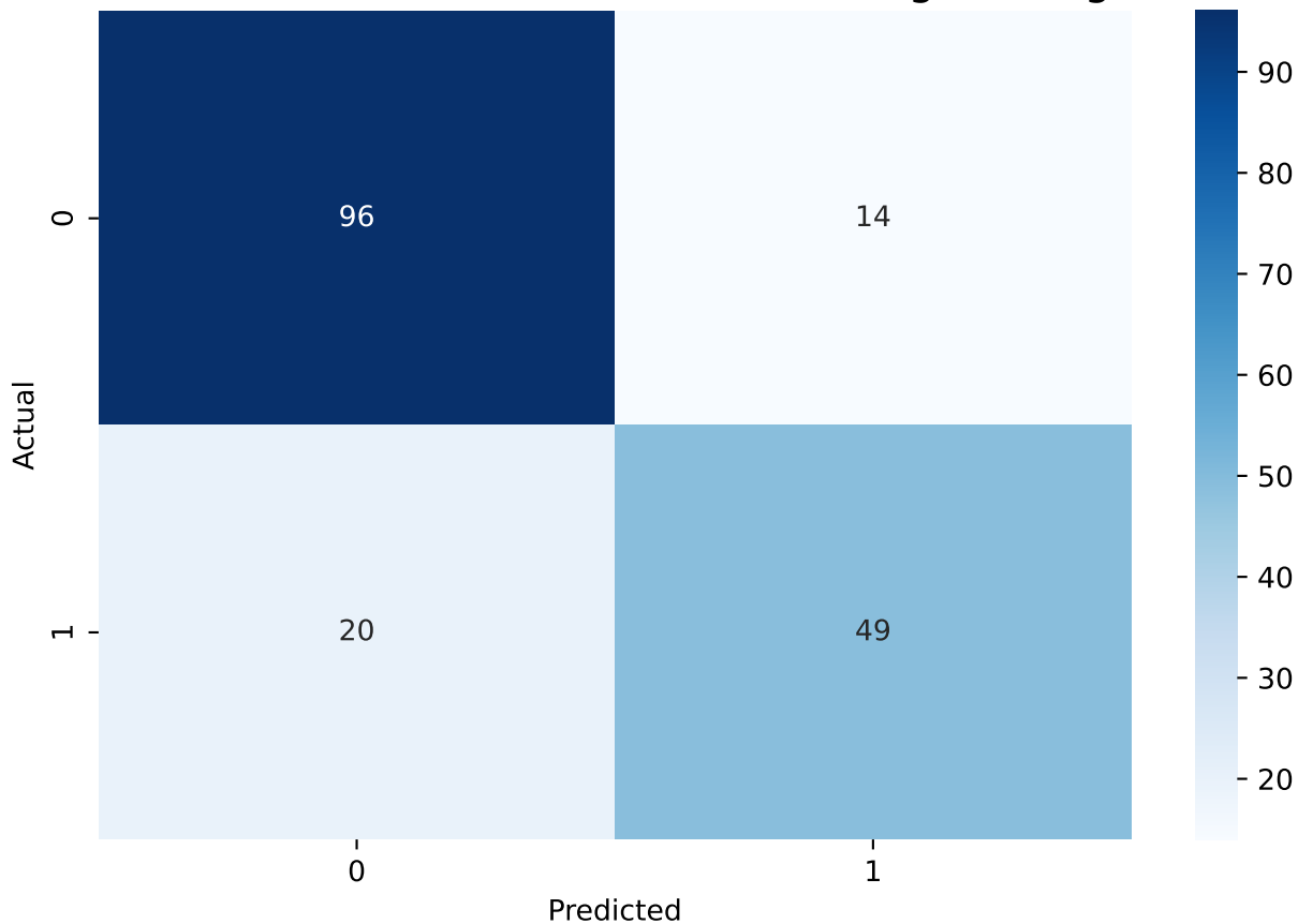
Confusion Matrix - Before Feature Engineering
