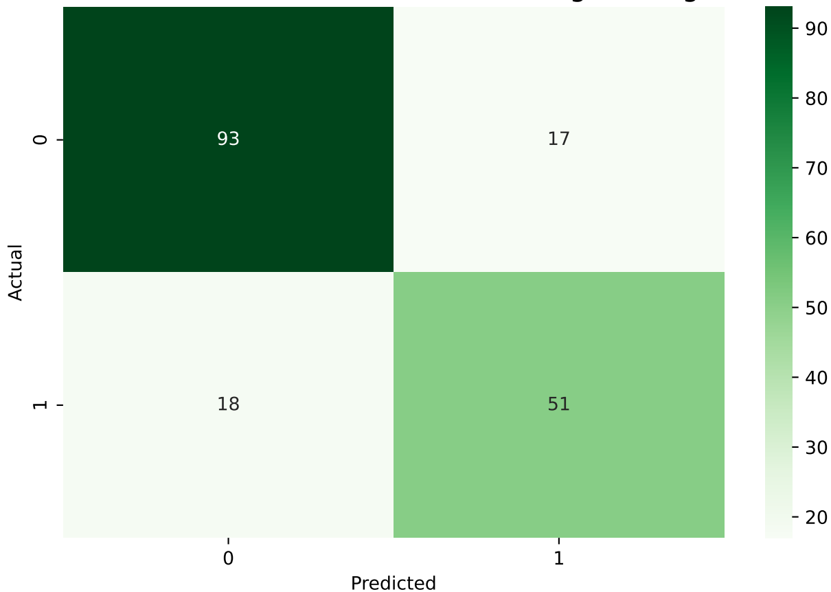
Confusion Matrix - After Feature Engineering
