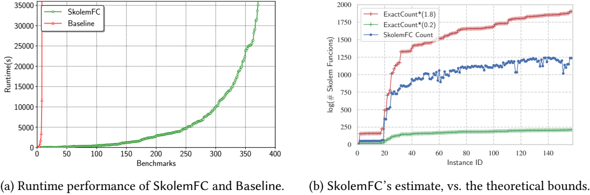
Figure 6.1: Performance and Correctness of SkolemFC
