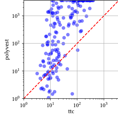
(b) Runtime comparison of ttc w.r.t. polyvest.
