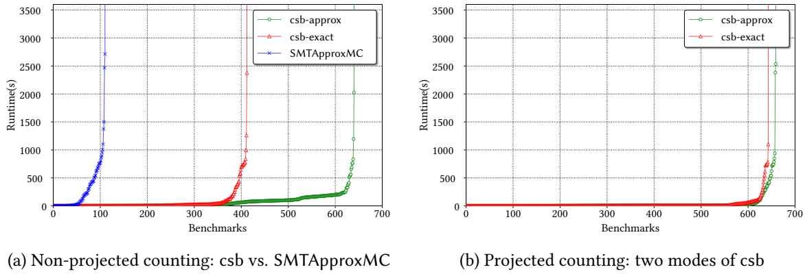
Figure 3.3: Performance of csb.
