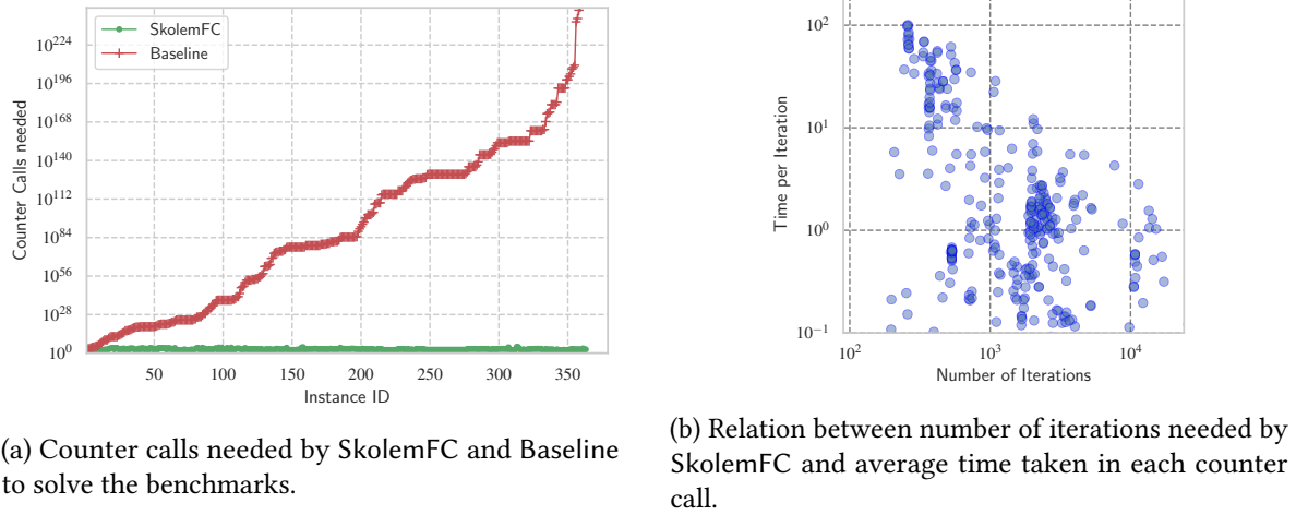
Figure 6.2: Coueter calls (iterations) and runtime.
