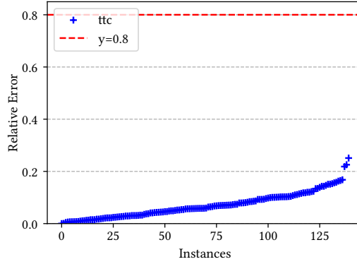
Figure 5.6: Quality of approximation: observed error.
