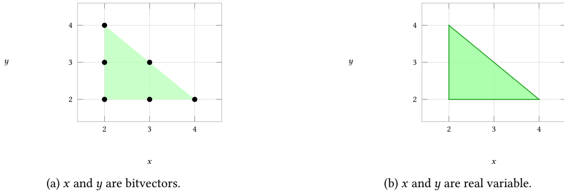
Figure 1.1: Solution space for same constraints in different theory.
