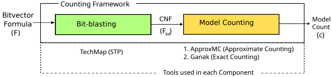
Figure 3.1: The architecture for counting in csb.
