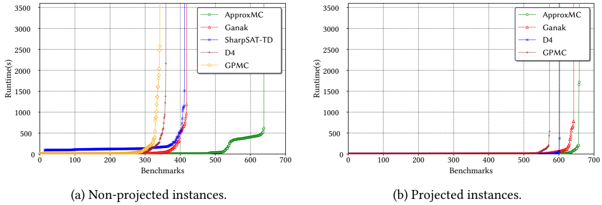
Figure 3.4: Performance comparison of model counters.
