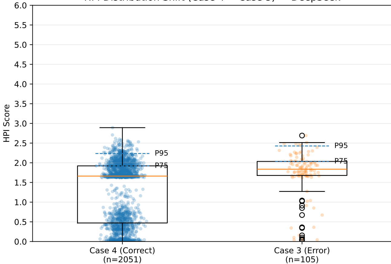
HPI Distribution Shift (Case 4 → Case 3) — DeepSeek
