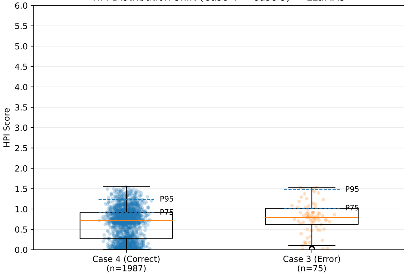
HPI Distribution Shift (Case 4 → Case 3) — LLaMA3
