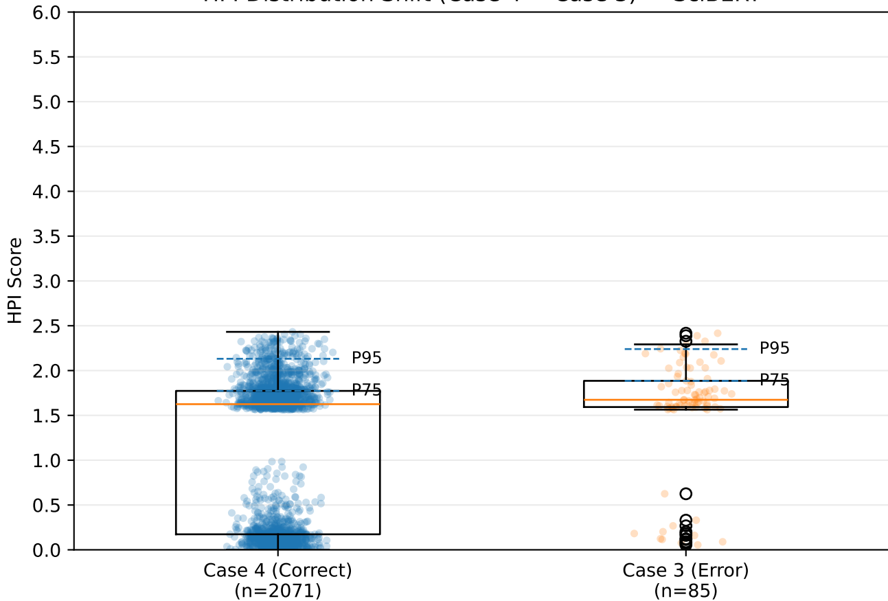
HPI Distribution Shift (Case 4 → Case 3) — SciBERT
