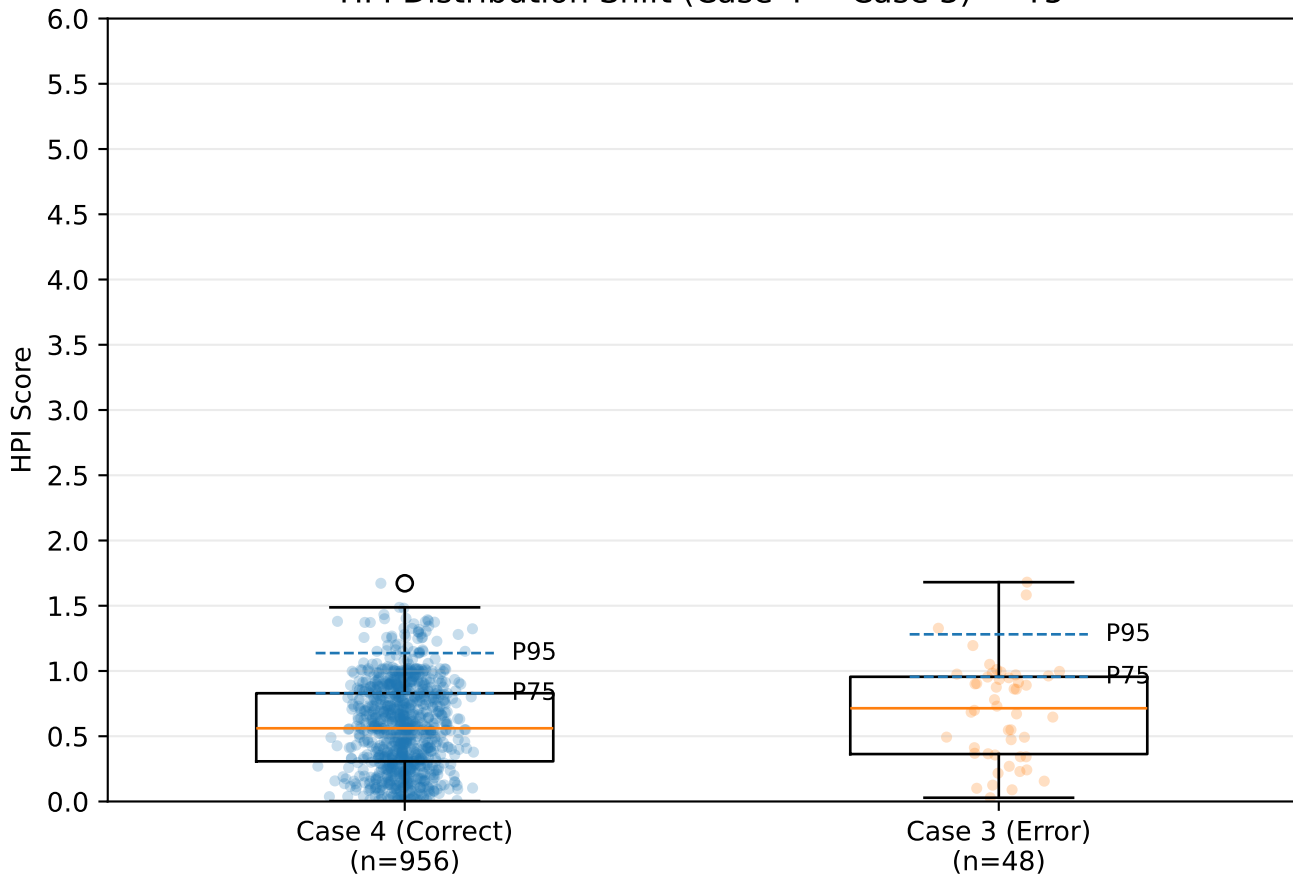
HPI Distribution Shift (Case 4 → Case 3) — T5
