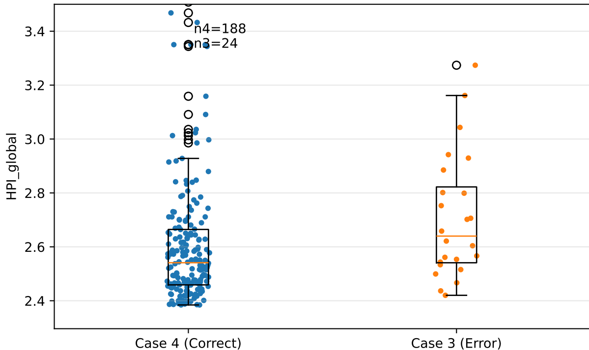
RoBERTa: Global HPI distribution (Case 4 vs Case 3)
